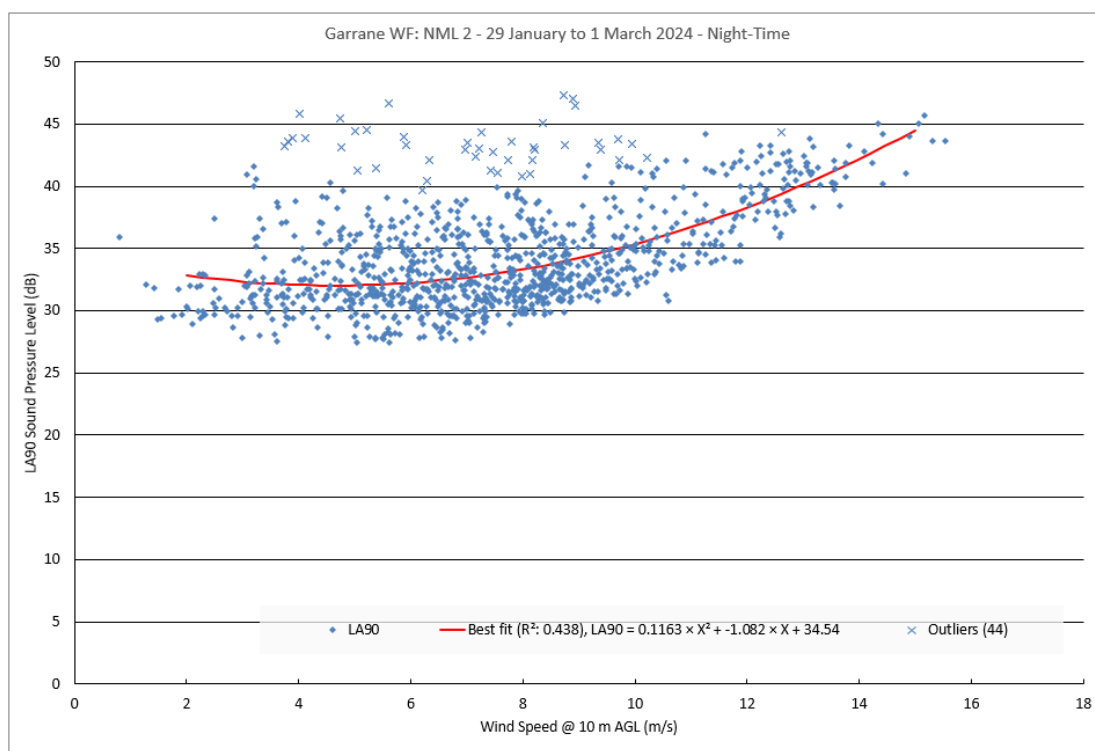
Chart 11.4: NML2 for night-time, background noise level, predicted level and assessment limit
