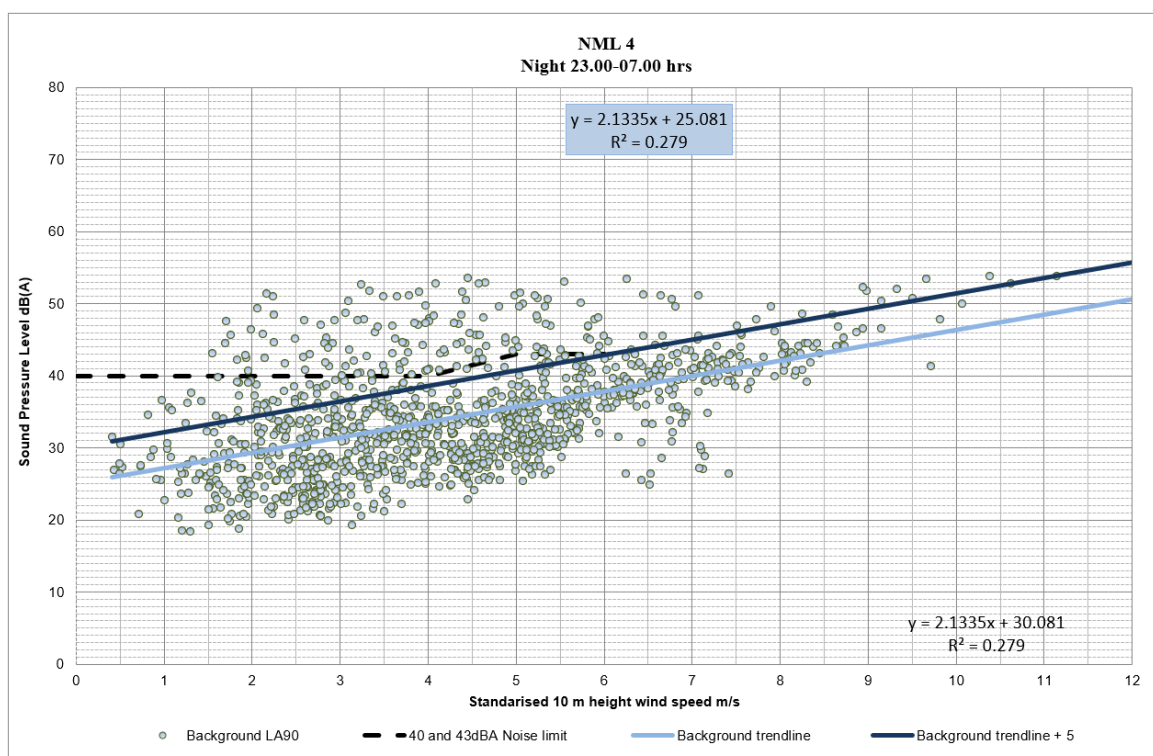
Chart 11.8: NML4 for night-time, background noise level, predicted level and assessment limit
