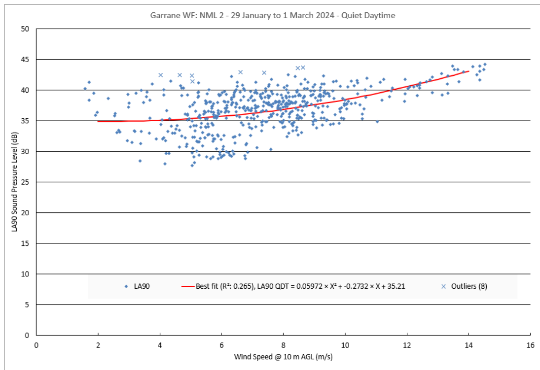
Chart 11.3: NML2 for quiet daytime, background noise level, predicted level and assessment limit
