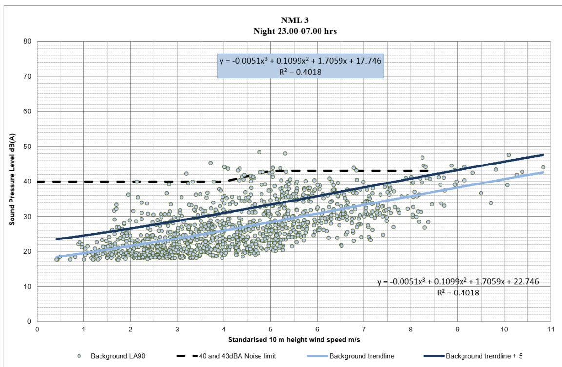
Chart 11.6: NML3 for night-time, background noise level, predicted level and assessment limit
