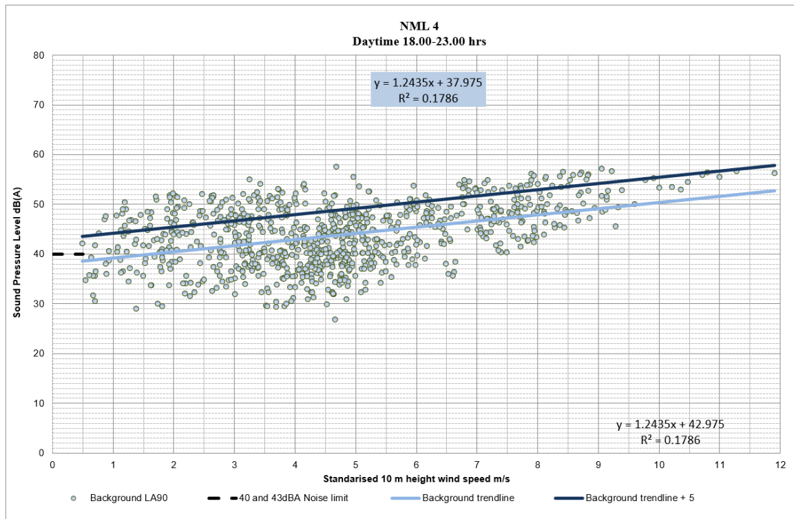
Chart 11.7: NML4 for quiet daytime, background noise level, predicted level and assessment limit
