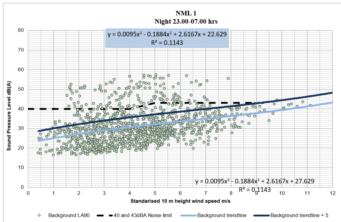
Chart 11.2: NML1 for night-time, background noise level, predicted level and assessment limit
