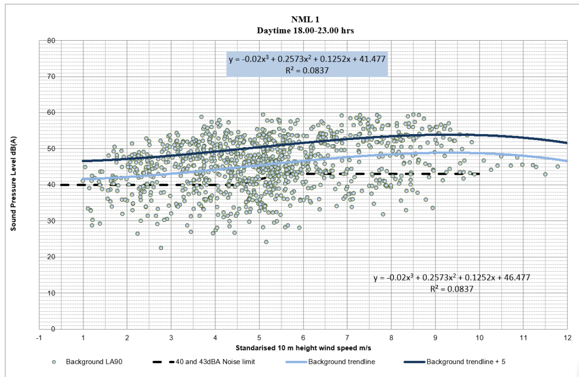
Chart 11.1: NML1 for quiet daytime, background noise level, predicted level and assessment limit
