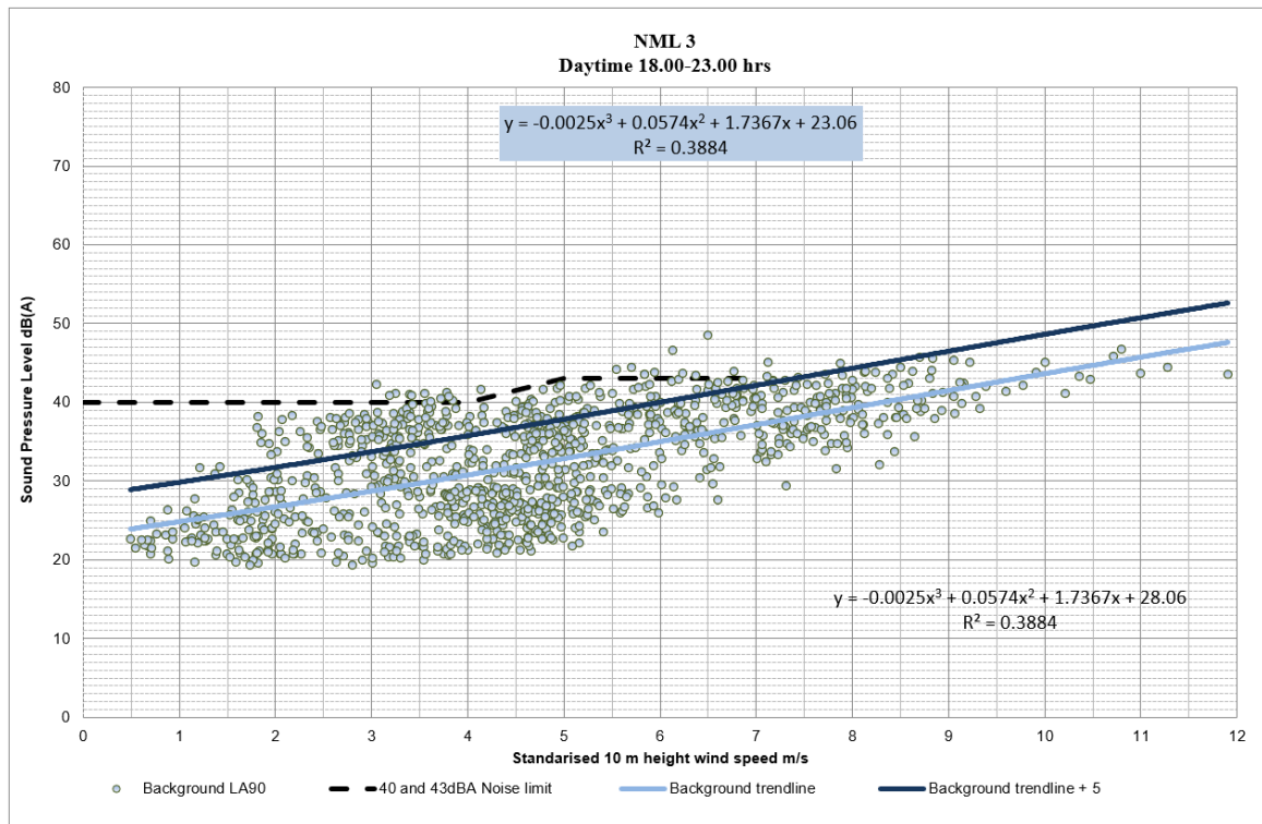
Chart 11.5: NML3 for quiet daytime, background noise level, predicted level and assessment limit
